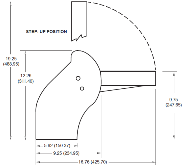
Side View
